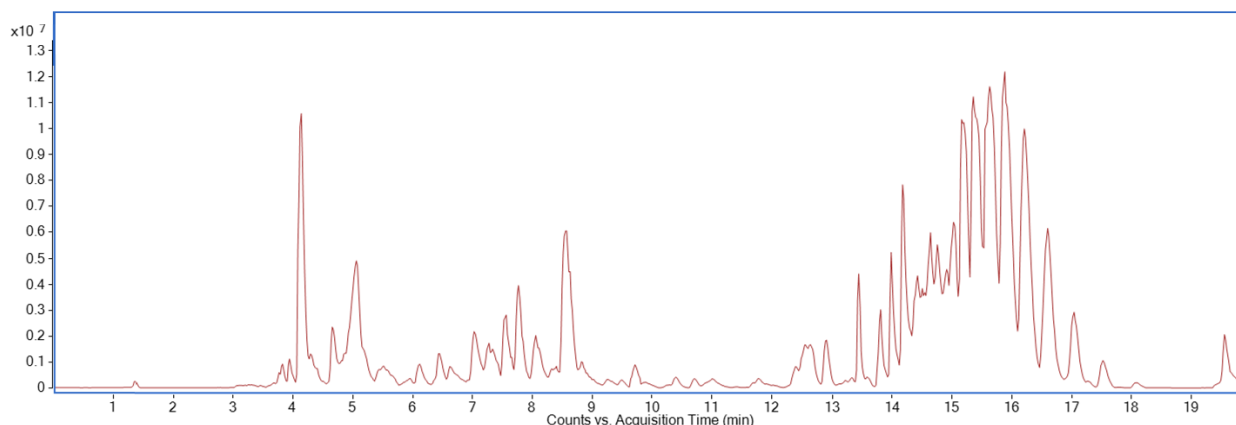
Figure 1: ML 2339/21 - UHPLC-HRMS/MS total compound chromatogram obtained for undiluted sample in ESI+
