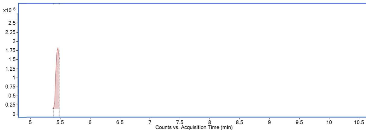
Figure 5: ML 2339/21 - UHPLC-HRMS/MS extracted ion chromatogram of 1 compound with unique combination of exact mass and RT detected in ESI+ (obtained for undiluted sample)
