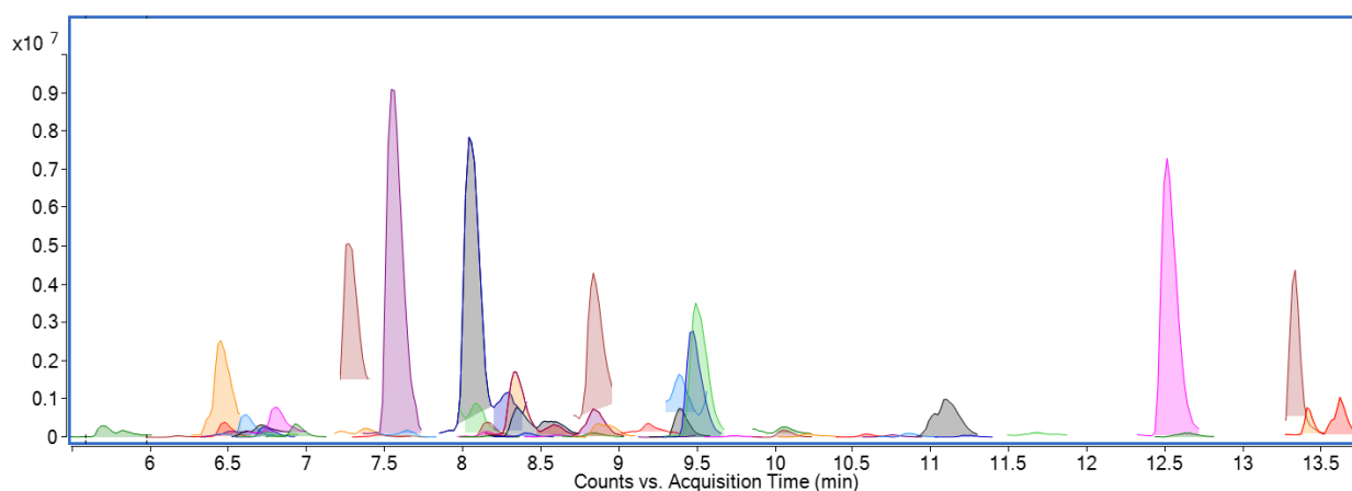
Figure 4: ML 2339/21 - UHPLC-HRMS/MS extracted ion chromatogram of 56 compounds with unique combination of exact mass and RT detected in ESI- (obtained for undiluted sample)
