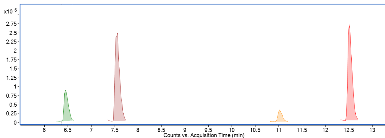
Figure 3: ML 2339/21 - UHPLC-HRMS/MS extracted ion chromatogram of 4 compounds with unique combination of exact mass and RT detected in ESI+ (obtained for undiluted sample)
