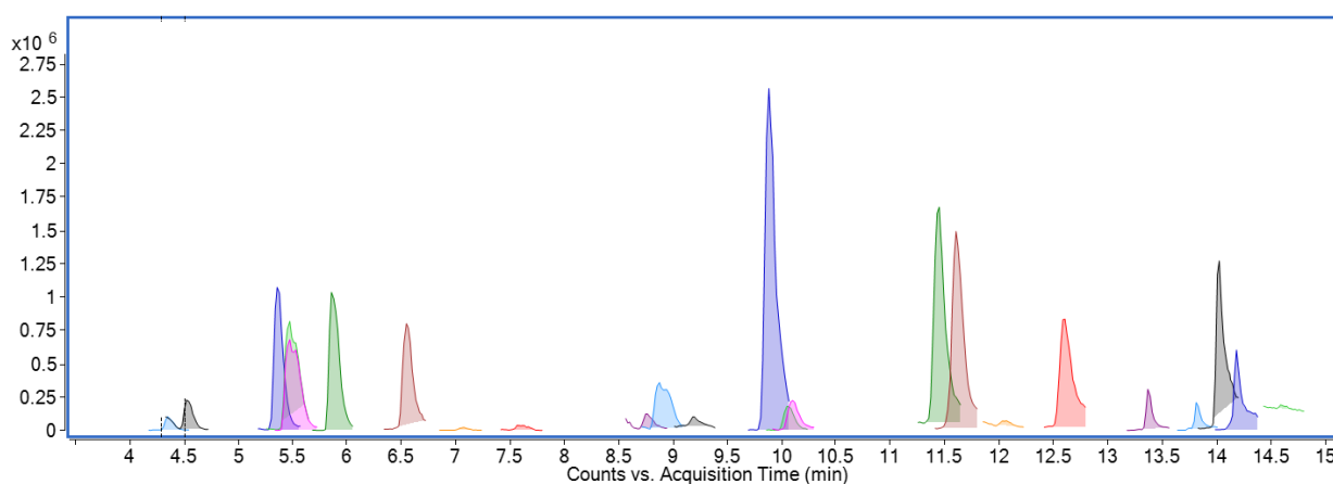
Figure 6: ML 2339/21 - UHPLC-HRMS/MS extracted ion chromatogram of 25 compounds with unique combination of exact mass and RT detected in ESI- (obtained for undiluted sample)
