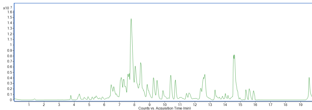
Figure 2: ML 2339/21 - UHPLC-HRMS/MS total compound chromatogram obtained for undiluted sample in ESI-
